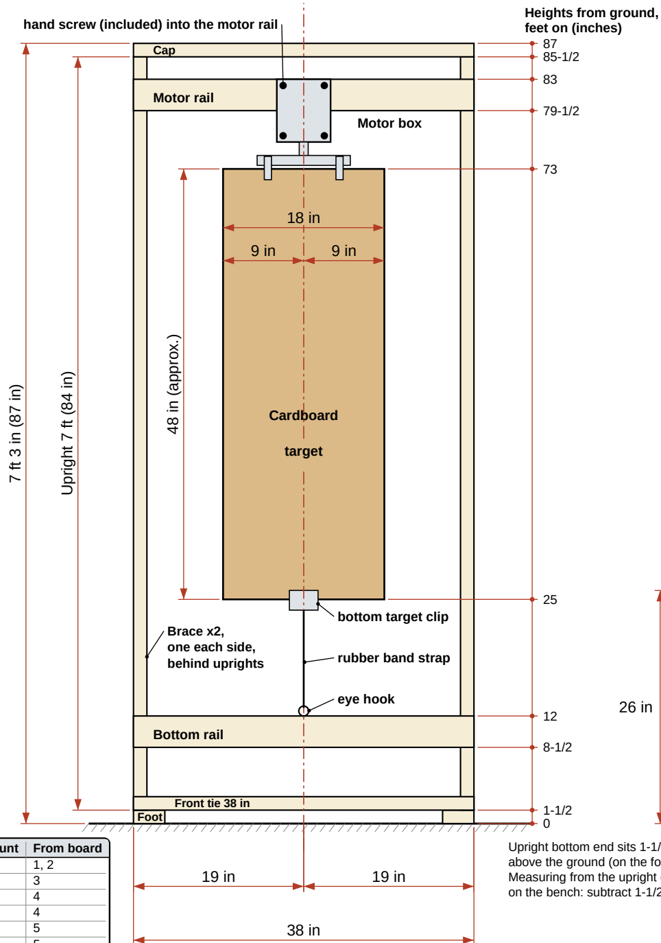
FRONT VIEW
